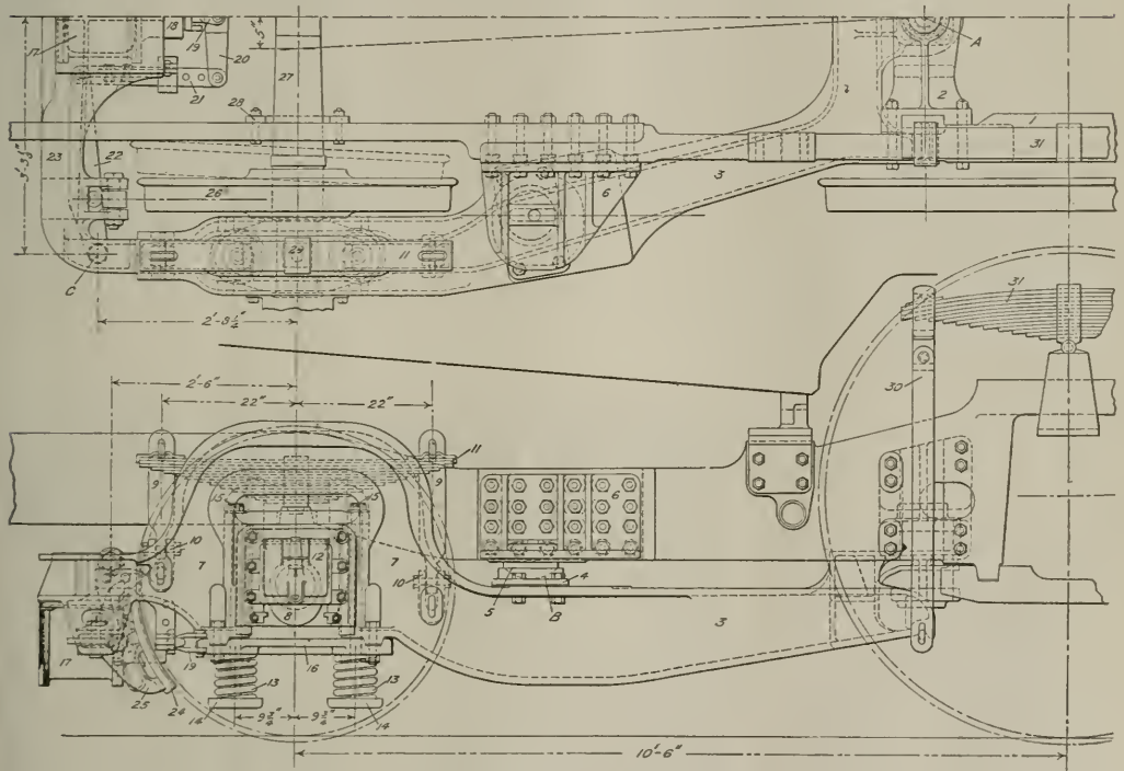
DETAILS OF TRAILING TRUCK.
